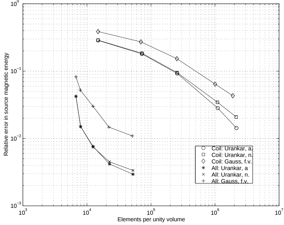
Figure 7: Comparison in logarithmic scale of relative errors in source magnetic energy
