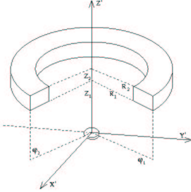
Figure 1: Circular coil with rectangular cross section
