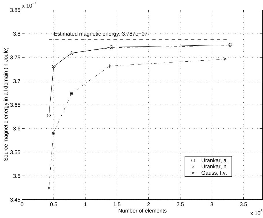
Figure 5: Trend of the source magnetic energy in free space (global domain)
