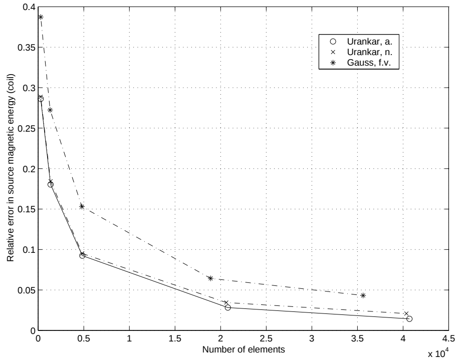
Figure 9: Relative errors of the source magnetic energy in free space (coil)
