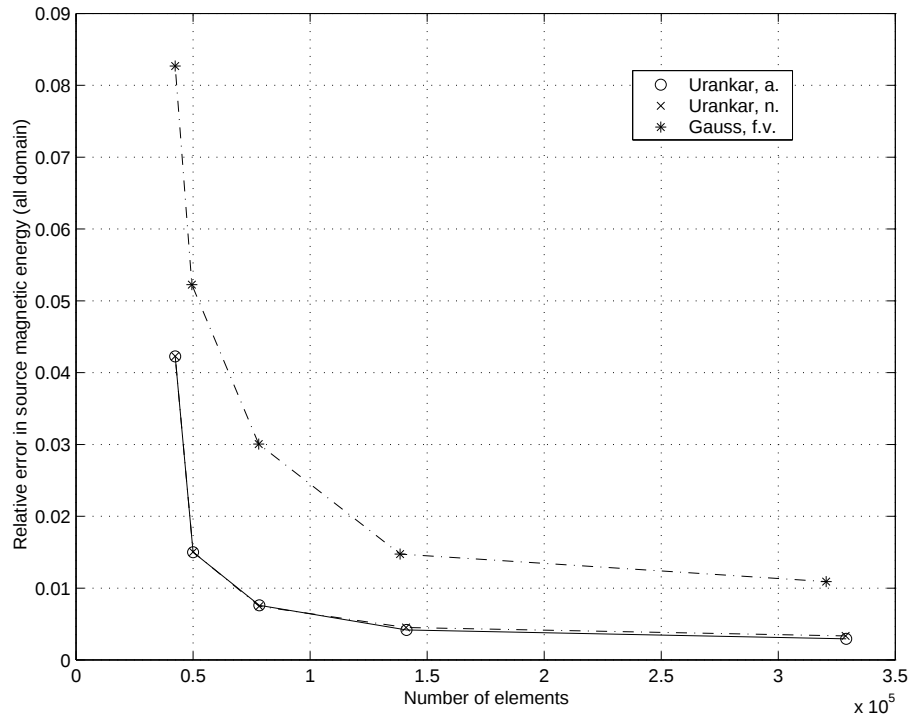
Figure 8: Relative errors of the source magnetic energy in free space (global domain)
