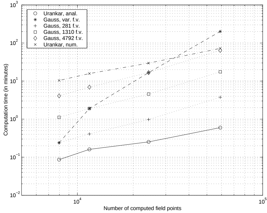
Figure 11: Trend of computational times in logarithmic scale
