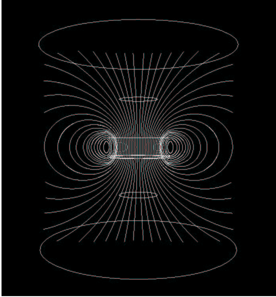
Figure 3: Streamlines of the magnetic field generated by a constant current in a circular coil with rectangular cross section
