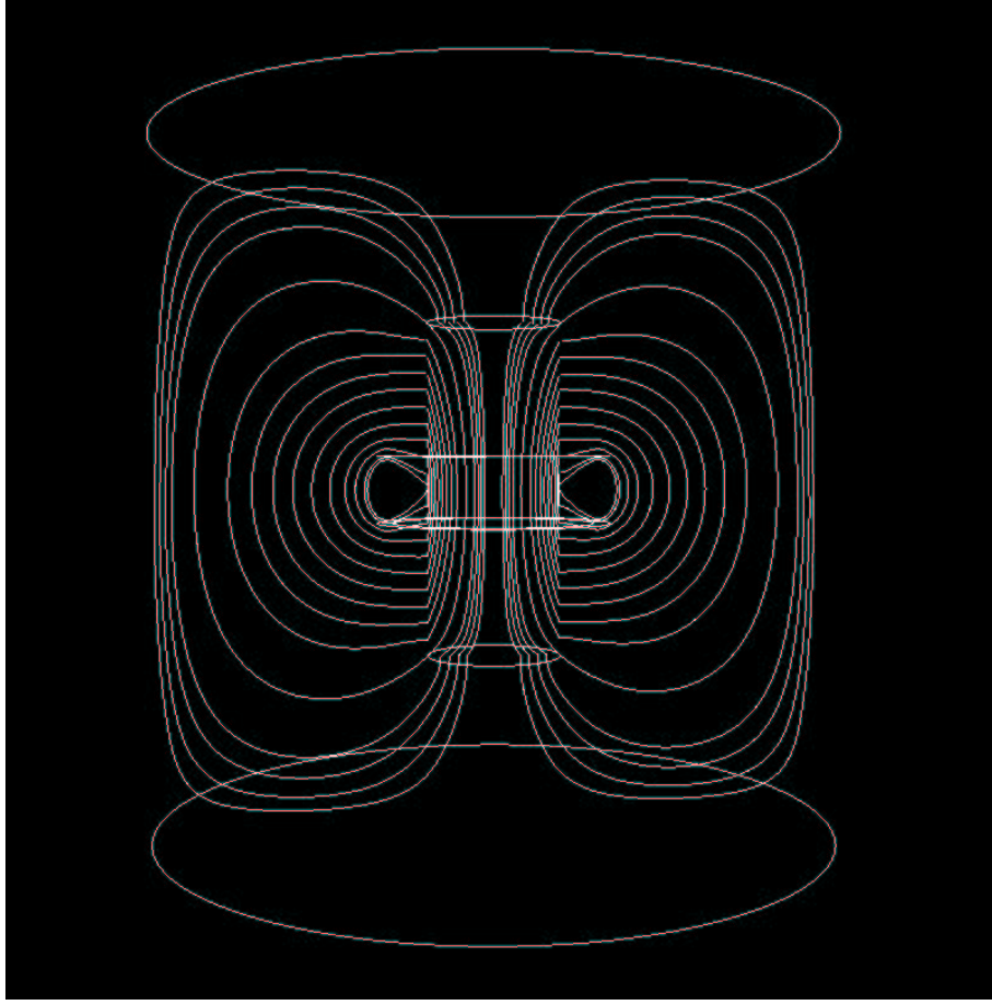
Figure 4: Streamlines of the total magnetic field in the material system iron/air associated to the test model
