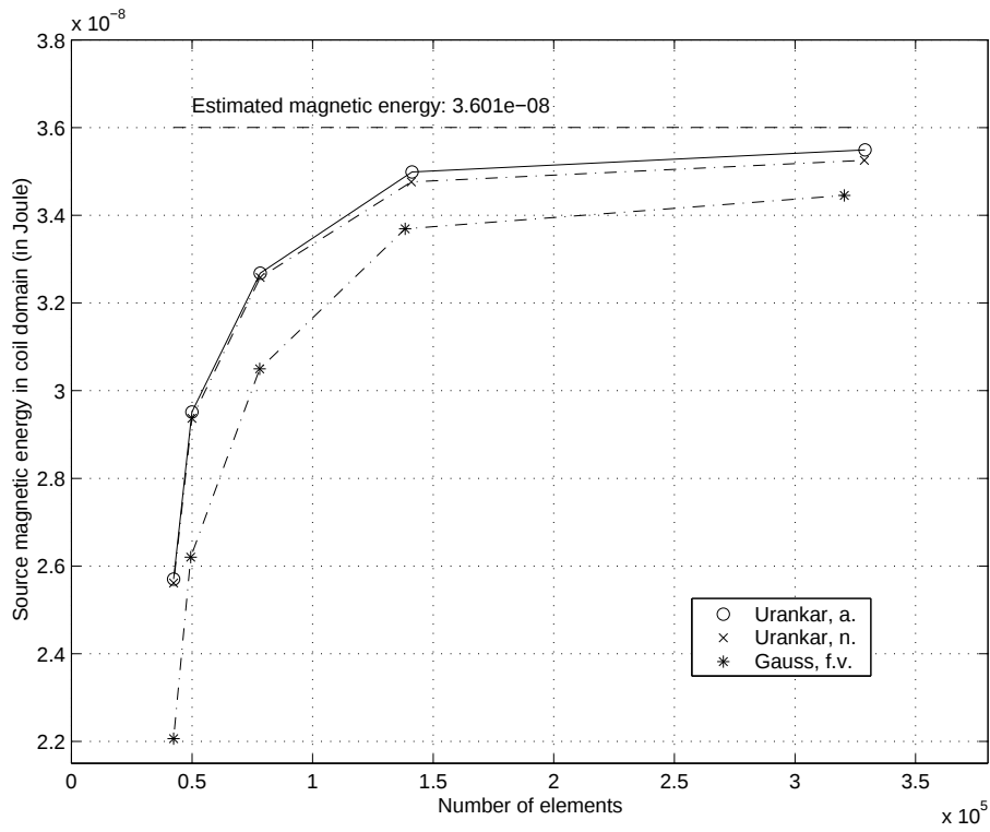
Figure 6: Trend of the source magnetic energy in free space (coil)
