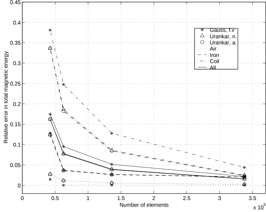
Figure 10: Comparison of relative errors in total magnetic energy among various materials
